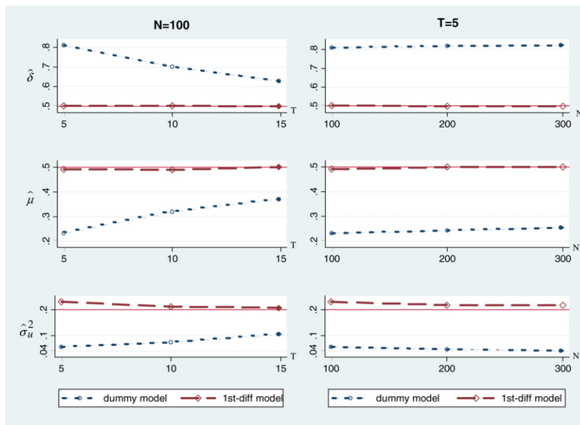
Fig. 1. Model comparisons.
